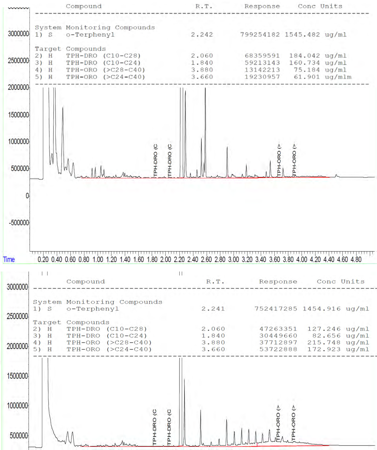
Figure D-17. 8015 Chromatograms of Sample DA59235-14 (Top) and the Respective Method Blank (Bottom)
